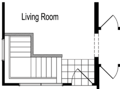
Opt. #2 Basement Plan
