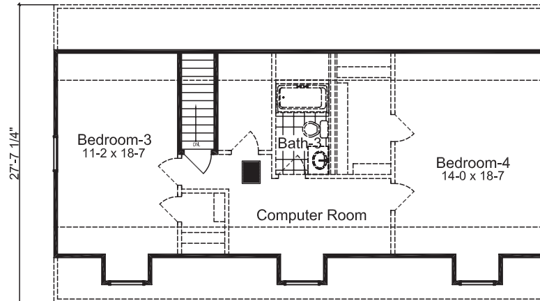
SECOND LEVEL FLOOR PLAN
